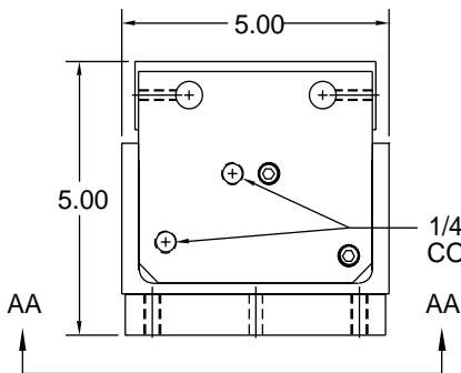
VIEW AA BOTTOM PLATE MOUNTING HOLES
