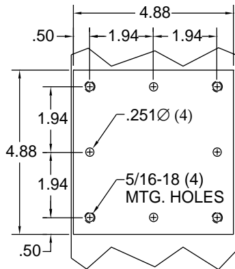
VIEW AA BOTTOM PLATE MOUNTING HOLES
