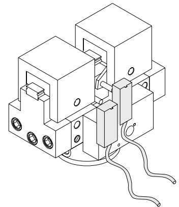
Proximity sensors preassembled for open & closed positions (see page 54)
