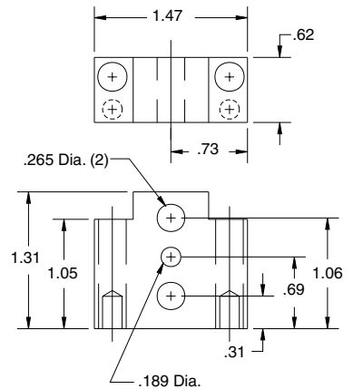
J1-2 jaw for B-2TPX (bolts & pins included)
